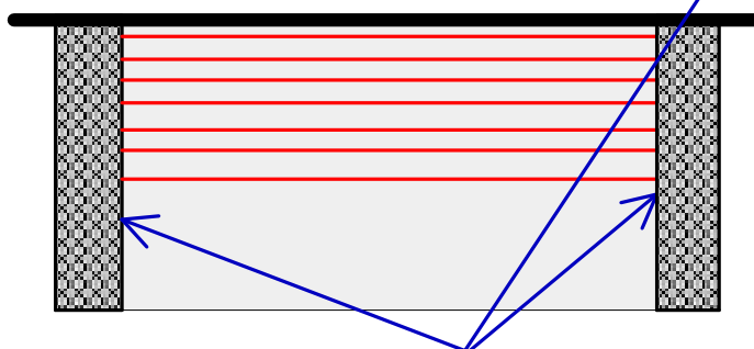
Rear view showing the battens (chequered) that offset the back of the box by 12mm from the wall, and the 2mm x 2mm grooves in the back of the box that give the bats places to grip on to when roosting / hibernating. Instead of grooves you may glue on wooden kebab skewers or ice-lolly sticks.
